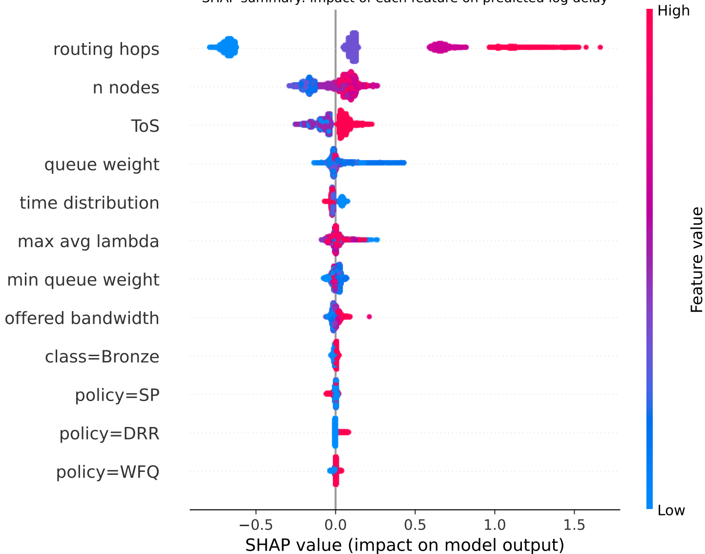
SHAP summary: impact of each feature on predicted log delay
